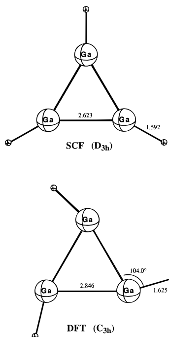
Figure 5. Optimized geometry (bond lengths in Å) for neutral (\text{GaH})_3 at the SCF TZ2P+diff and DFT TZ2P+diff levels of theory. This stationary point is not a minimum.
